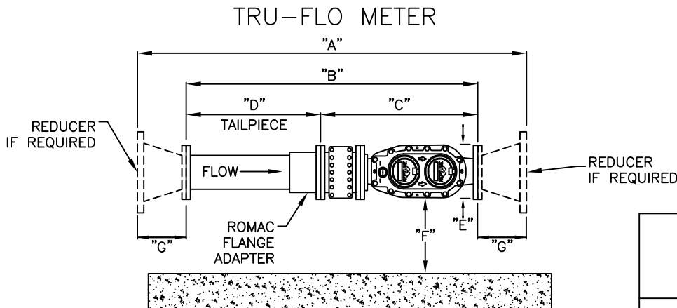
METER DIMENSIONAL DATA NTS
